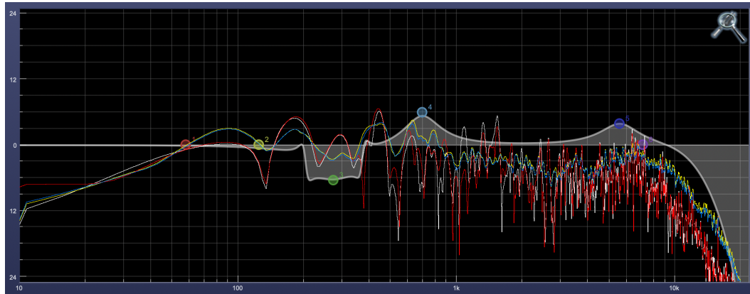
Spectrgraph Display
